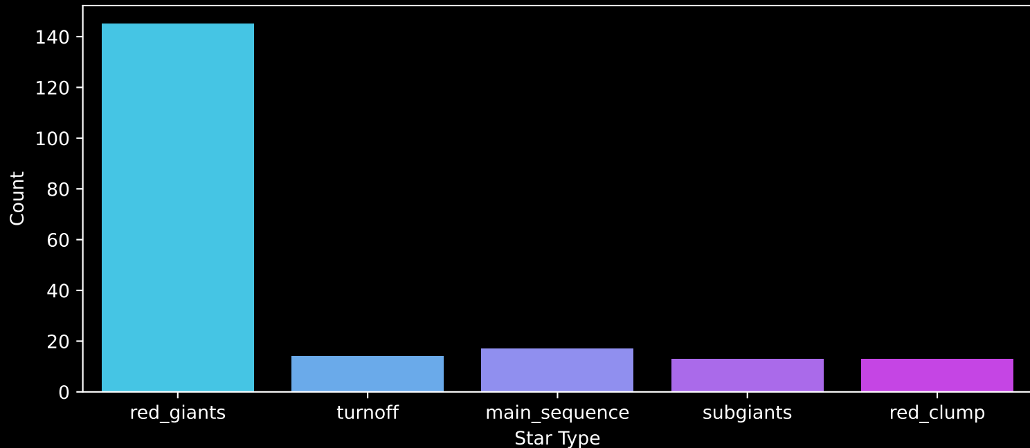
APOGEE DR17 Field: [199-04] Count plot of Star Type
