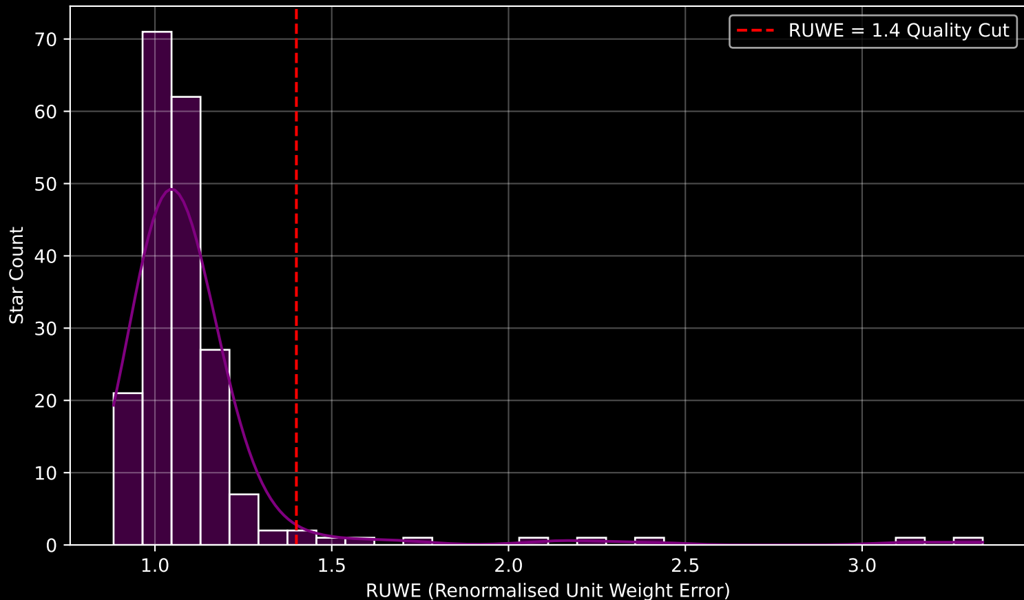
GAPOGEE DR17 Field [199-04] RUWE Distribution (n= 200)
