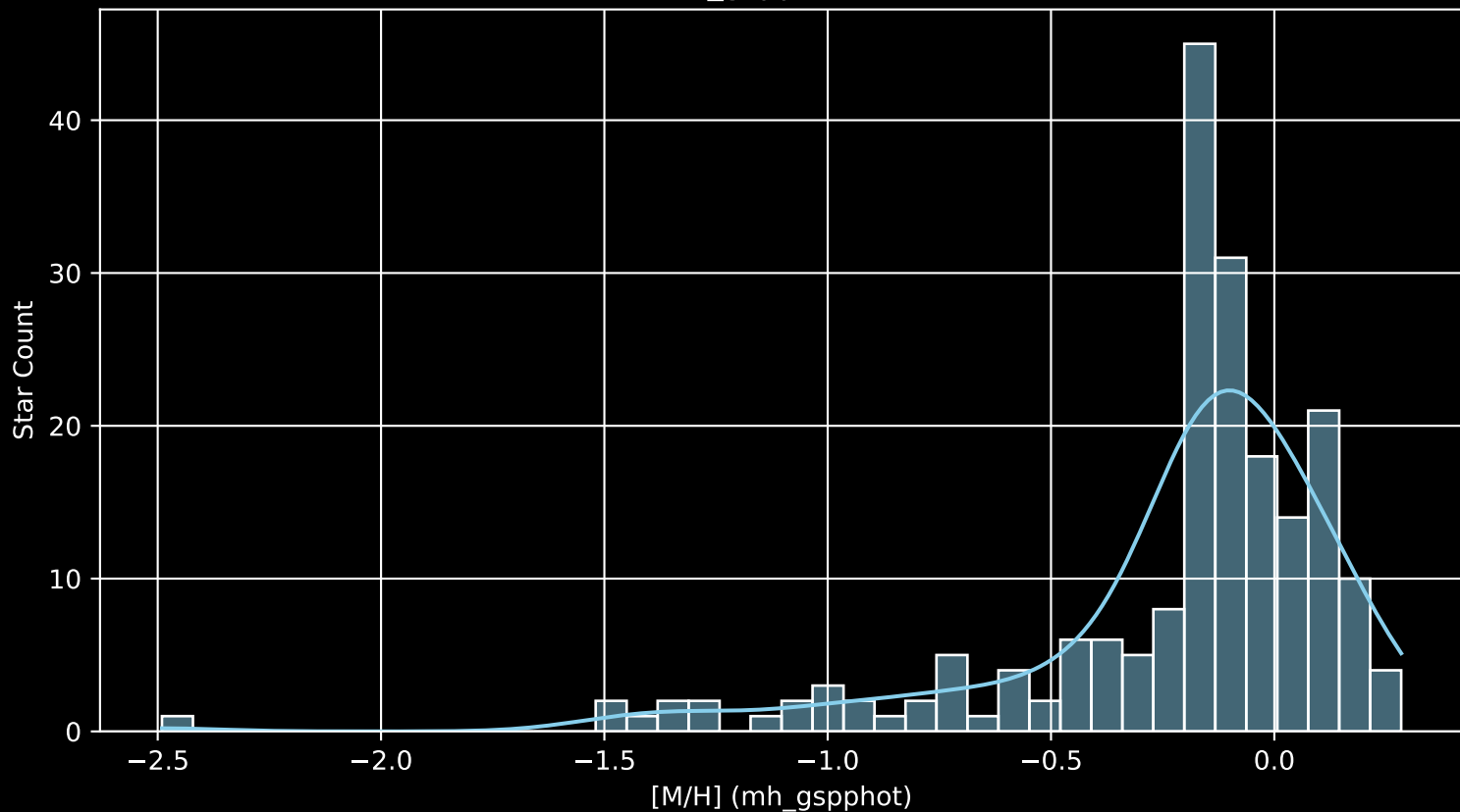
APOGEE DR17 Field: [199-04 [M/H] (mh_gspphot) (n= 199)
