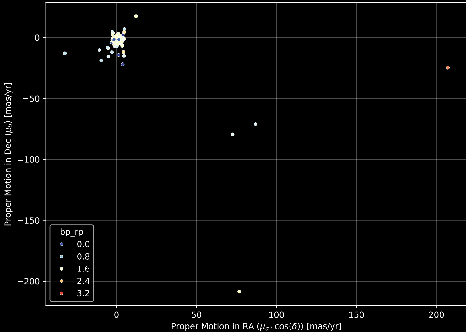
APOGEE DR17 Field: [199-04] Proper Motion Diagram (n= 202)
