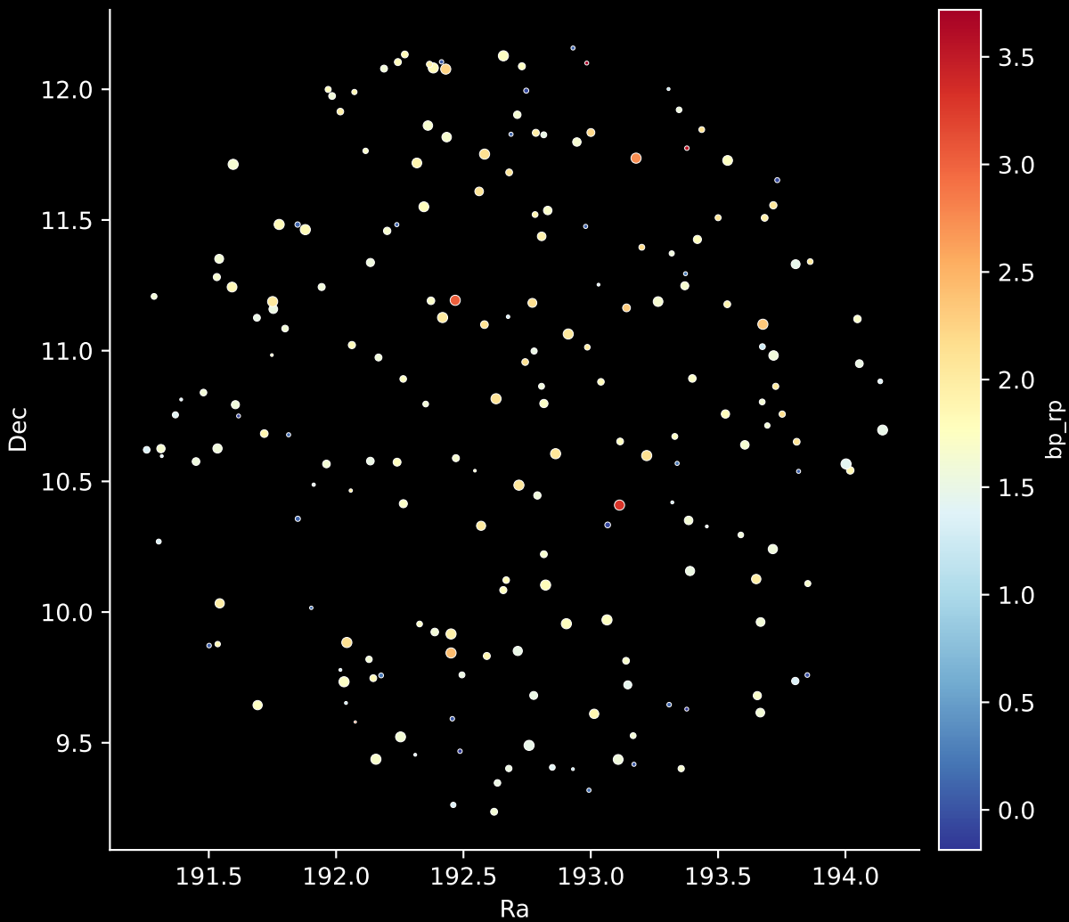
APOGEE DR17 Field: [199-04] Stars: 202
