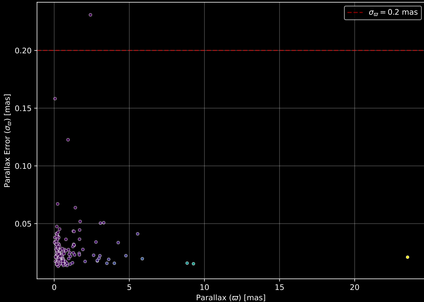
APOGEE DR17 Field: [199-04] Parallax Quality (n= 202)
